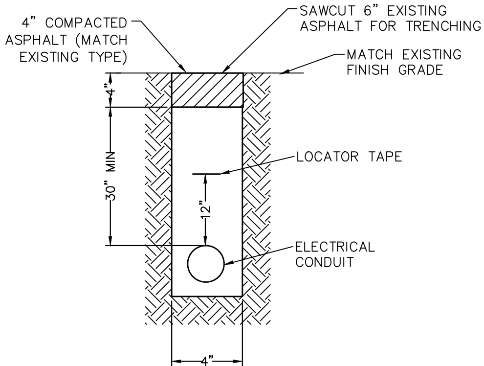
ELECTRICAL CONDUIT UNDER ROADWAY N.T.S (TYP.)
