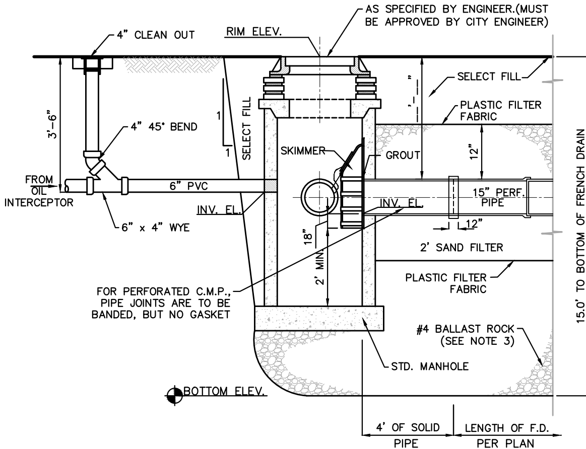
TYPICAL SECTION OIL INTERCEPTOR N.T.S.
