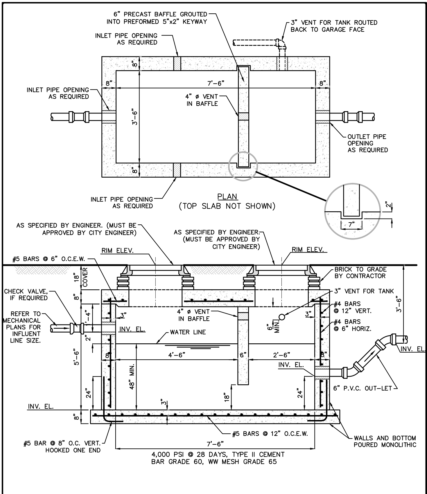
TYPICAL SECTION OIL INTERCEPTOR N.T.S.
