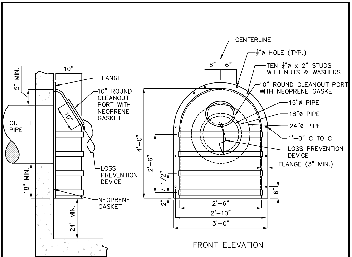
SIDE ELEVATION
