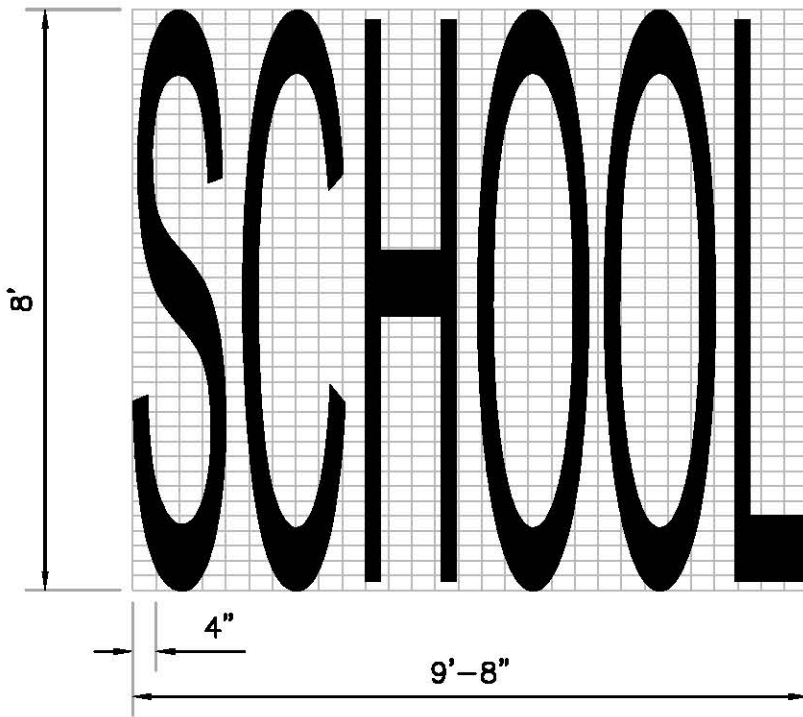
SINGLE-LANE PAVEMENT MARKING
