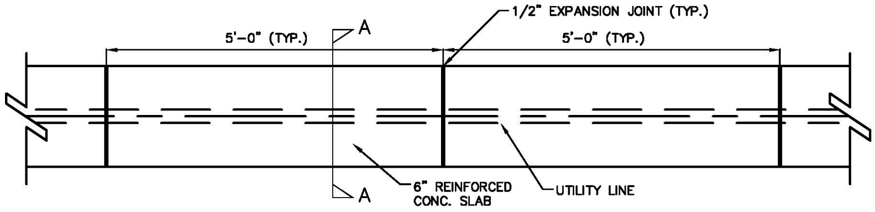
TYPICAL PAVEMENT RESTORATION OVER UTILITY LINE N.T.S.
